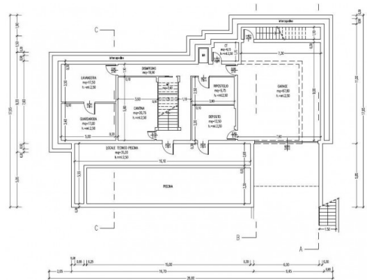
PIANO INTERRATO
